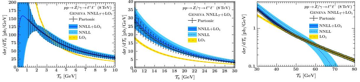
Figure 3: The GENEVA partonic results for Drell-Yan production, compared to the analytic resummation of T_0 matched to fixed order at NNLL+LO 1 , in the peak (left), transition (center), and tail (right) regions.
