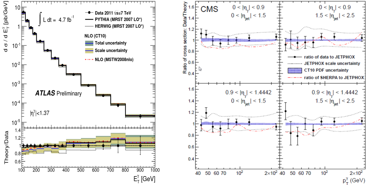
Figure 1: Left: Measured (dots with error bars) and expected inclusive prompt photon cross section in the ATLAS barrel \eta region 10 . The inner error bars on the data points show statistical uncertainties, while the full error bars show statistical and systematic uncertainties added in quadrature. The next to leading order theory prediction is shown as a shaded band which indicates theoretical uncertainties, while the leading order parton shower Monte Carlo generators are shown as lines. Right: The ratios of the photon-jet triple-differential cross section to the NLO QCD prediction using JETPHOX with the CT10 PDF set and scales, as measured by CMS 16 with 2.14 \text{ fb}^{-1} . Errors show the statistical and systematic uncertainties added in quadrature. The two dotted lines represent the effect of varying the theoretical scales. The shaded region is the CT10 PDF uncertainty. The dash-dotted lines show the ratios of the SHERPA predictions to JETPHOX.
