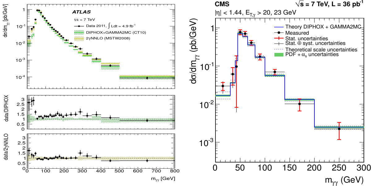
Figure 2: Left: Comparison between the ATLAS experimental cross sections and the predictions obtained with DIPHOX+GAMMA2MC (NLO) and 2 \gamma NNLO (NNLO) for the di-photon invariant mass 20 . The black dots correspond to data with with error bars for their total uncertainties, which are dominated by the systematic component. The theoretical uncertainties include contributions from the limited size of the simulated sample, from the renormalization and factorization scales choice and from uncertainties on the parton distribution functions and on the hadronization and underlying event corrections. Right: Measured cross section of di-photon production as a function of the invariant mass of the photon pair for photons within the pseudorapidity region |\eta| < 1.44 , as seen by CMS 19 . The inner and outer error bars on each point show the statistical and total experimental uncertainties. The 4% uncertainty on the integrated luminosity is not included in the error bars. The dotted line and shaded region represent the systematic uncertainties on the theoretical prediction from the theoretical scales and the PDFs, respectively.
